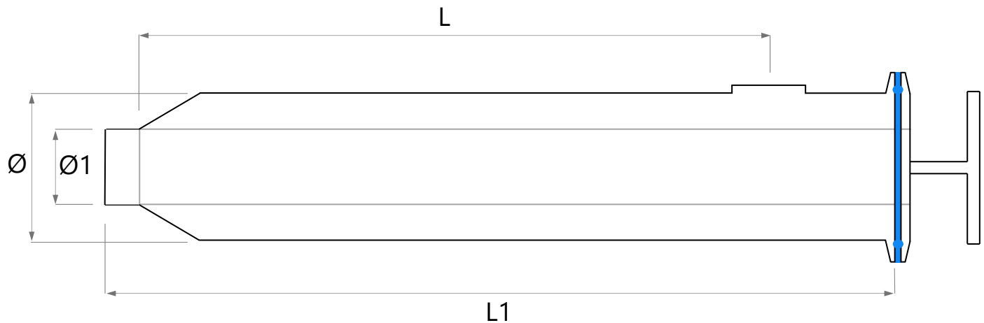
TYPE B 90° PRODUCT STRAINER BODY 316L
