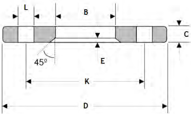
PN16 BACKING FLANGES - TABLE D THICK - ZINC PLATED & 304 ST/ST
