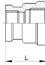
BSP REDUCING SOCKET 316
